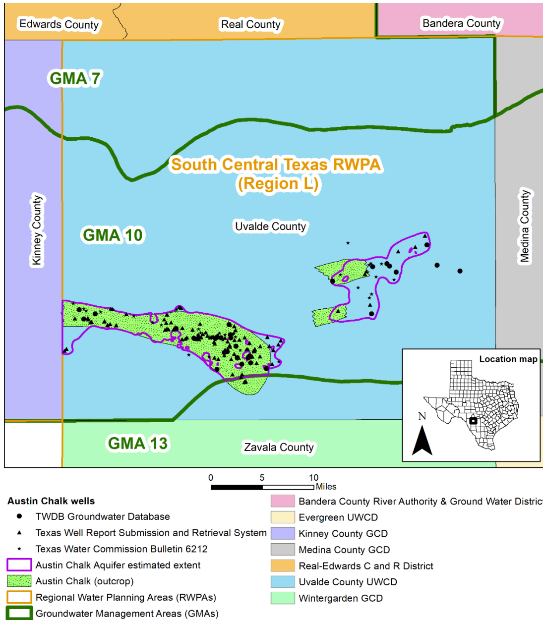
FIGURE 1. REGIONAL WATER PLANNING AREAS (RWPAS), GROUNDWATER MANAGEMENT AREAS (GMAS), GROUNDWATER CONSERVATION DISTRICTS (GCDs, UWCD), AND COUNTIES IN THE VICINITY OF THE AUSTIN CHALK AQUIFER IN UVALDE COUNTY (MODIFIED FROM BRADLEY AND BOGHICHI, 2018).
