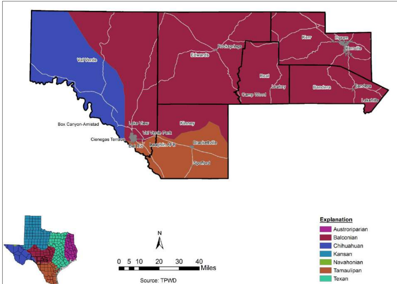
Figure 1-8. Biotic Provinces
